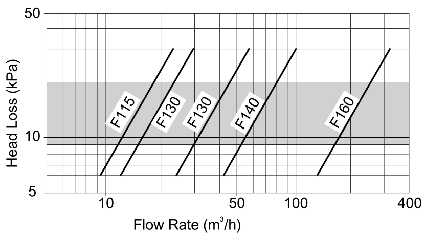
RMS 100 - Head Loss Graph
