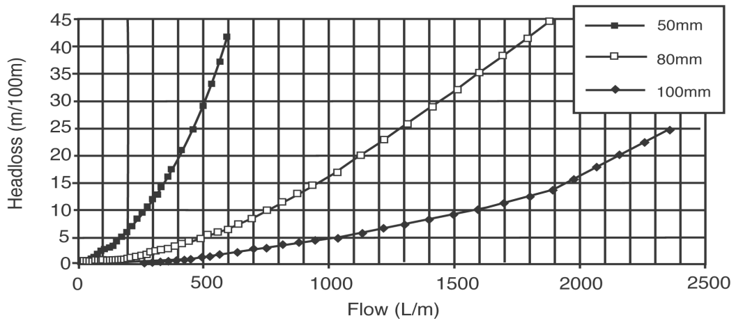
Friction Loss Chart
