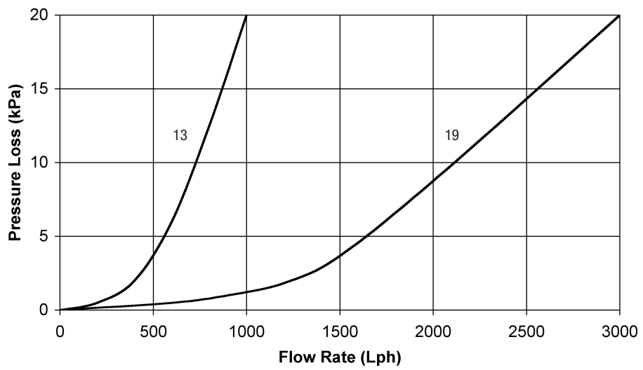
Pressure Loss vs Flow 13 and 19mm Filter
