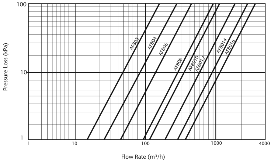
Head Loss Graph (120 mesh)
