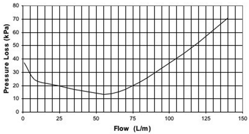
Flow vs Pressure Loss
