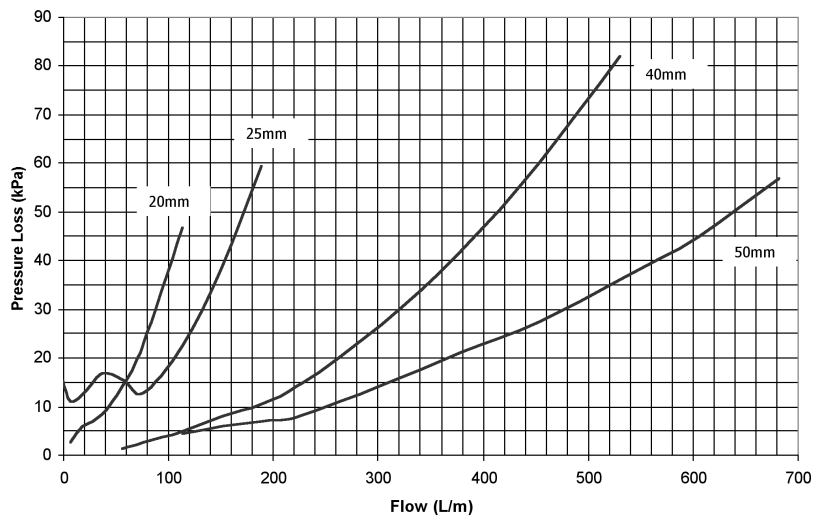
Flow vs Pressure Loss
