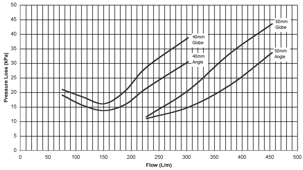
Flow vs Pressure Loss
