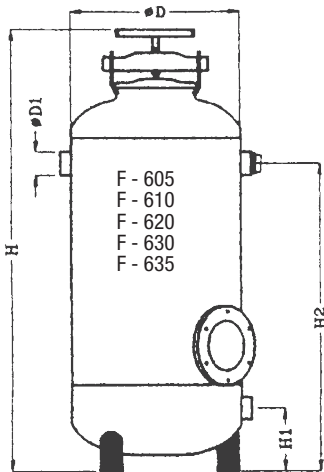
PVT Tank DIMENSIONAL DRAWINGS
