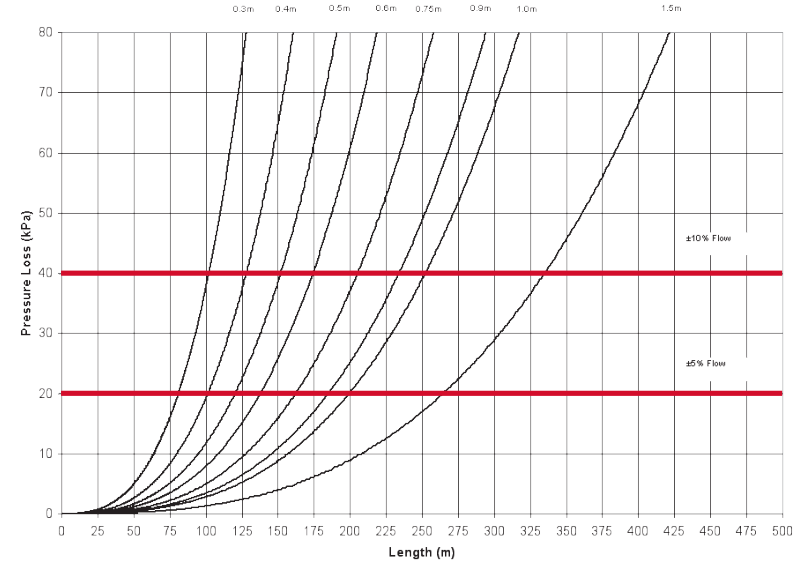
20mm Drip-In Classic 2.5 L/h Run Length (m) vs Pressure Loss (kPa)
