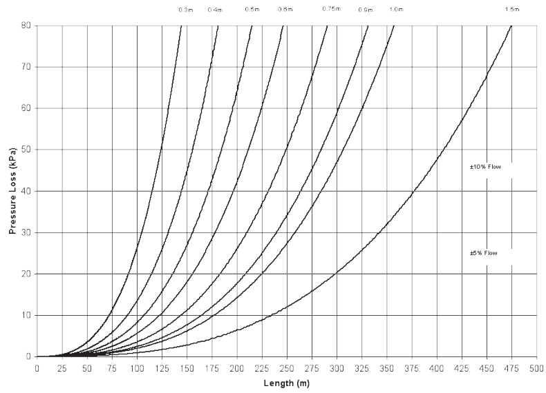
20mm Drip-In Classic 2.0 L/h Run Length (m) vs Pressure Loss (kPa)
