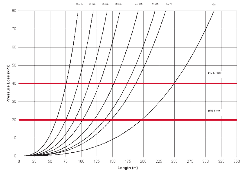
20mm Drip-In Classic 4.0 L/h Run Length (m) vs Pressure Loss (kPa)
