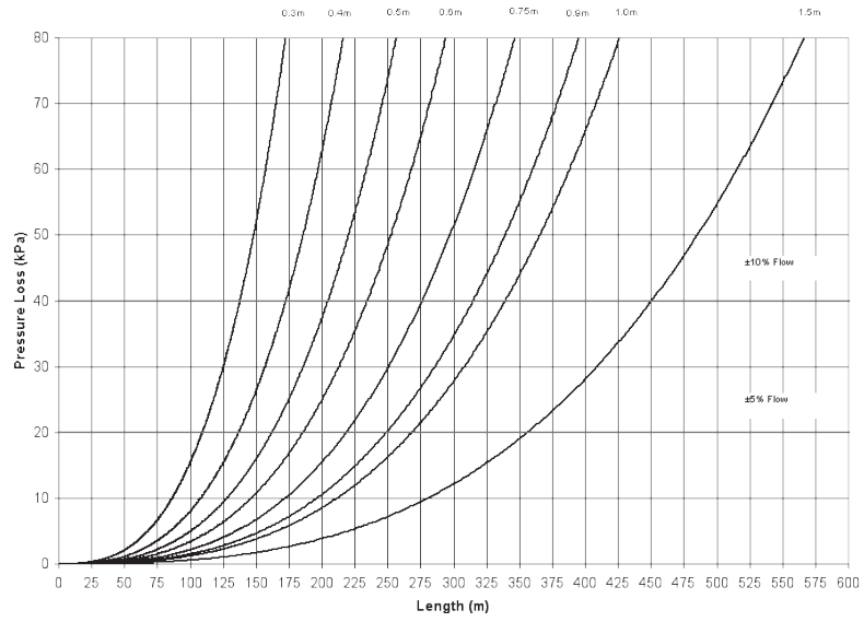
20mm Drip-In Classic 1.6 L/h Run Length (m) vs Pressure Loss (kPa)
