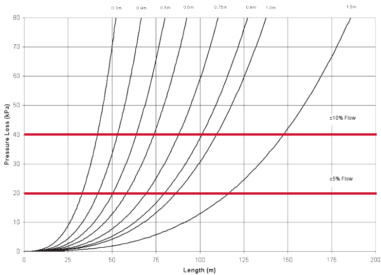
16mm Drip-In Classic 4.0 L/h Run Length (m) vs Pressure Loss (kPa)
