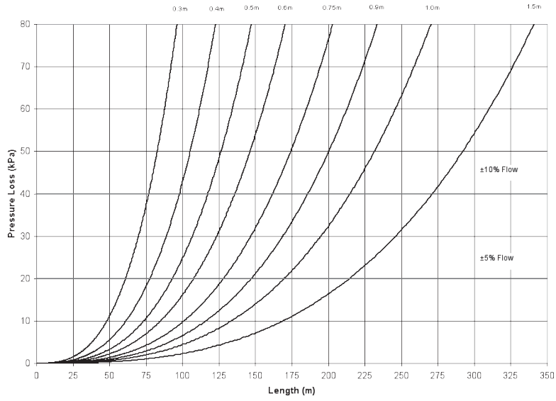
16mm Drip-In Classic 1.6 L/h Run Length (m) vs Pressure Loss (kPa)
