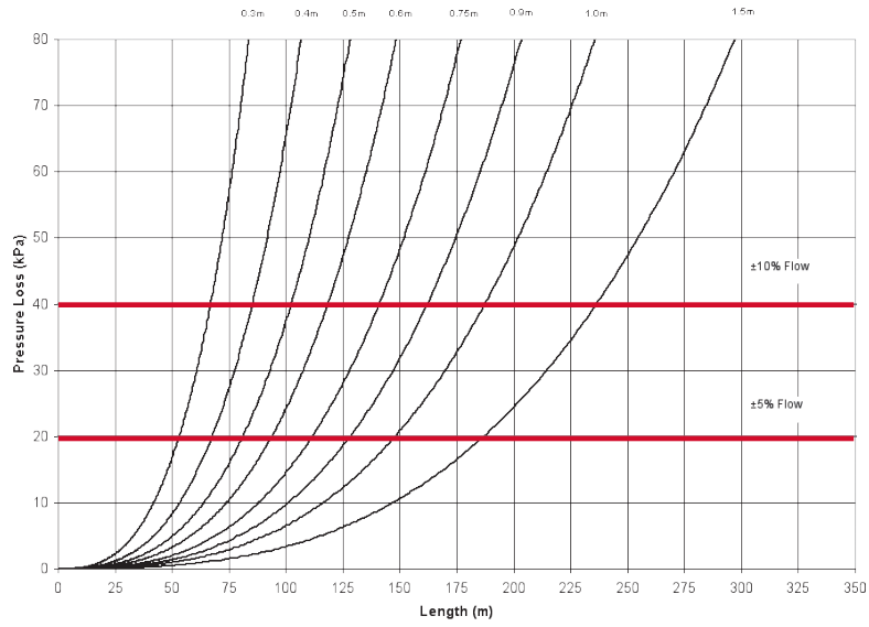
16mm Drip-In Classic 2.0 L/h Run Length (m) vs Pressure Loss (kPa)
